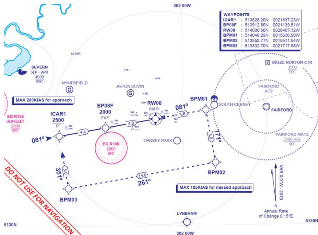
Airspace Chart - RNP ARCH RWY08
