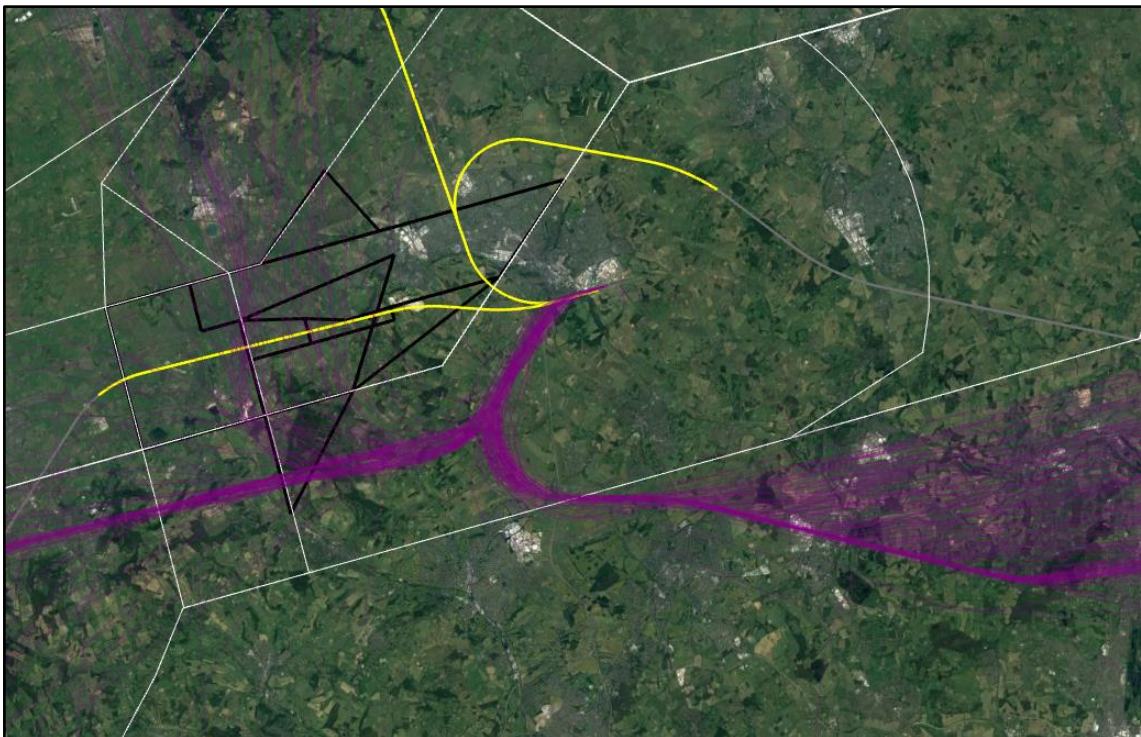
Figure 32: Existing departure swaths (purple) and W SID Group 7 Period 2 illustrative centrelines (yellow) from Luton's westerly runway
