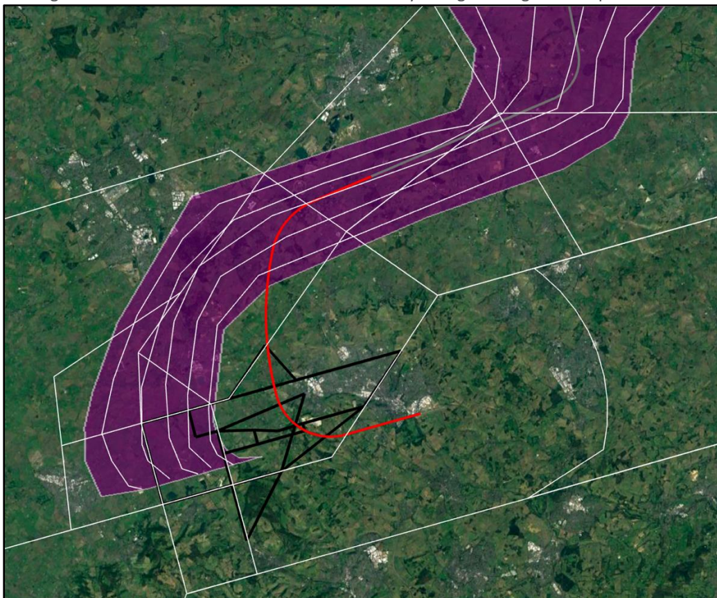
Figure 49: Easterly arrival swath moved North (purple) and RNP-AR arrival route in red
