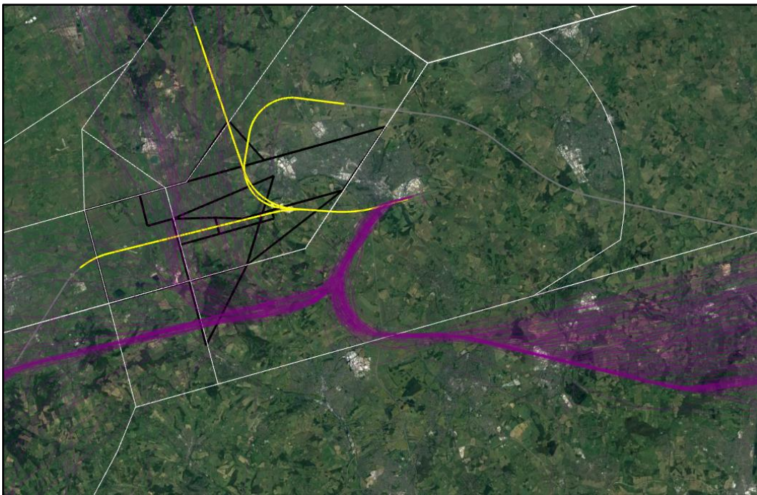
Figure 34: Existing departure swaths (purple) and W SID Group 8 Period 1 illustrative centrelines (yellow) from Luton's westerly runway
