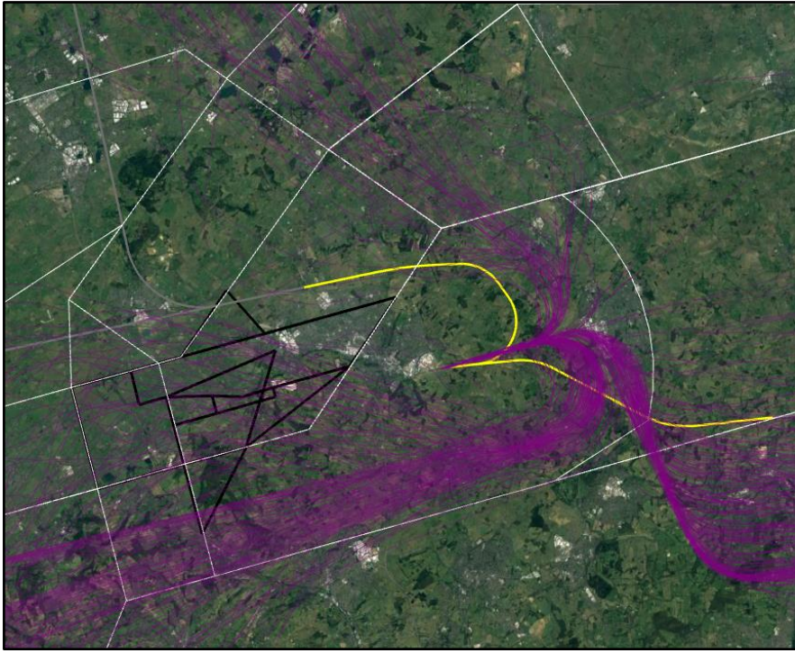
Figure 40: Existing departure swaths (purple) and the E SID Group 6 Period 1 illustrative centrelines (yellow) from Luton's Easterly runway
