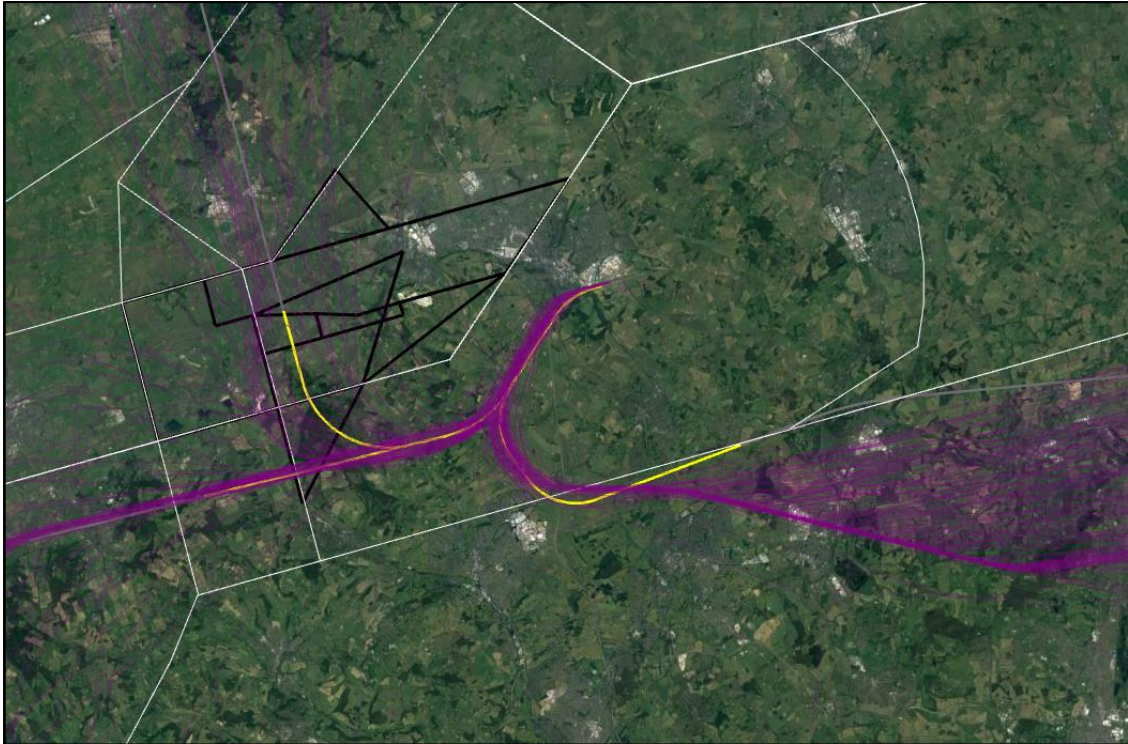
Figure 31: Existing departure swaths (purple) and W SID Group 7 Period 1 illustrative centrelines (yellow) from Luton's westerly runway
