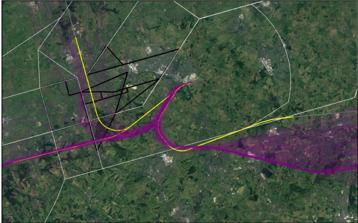
Figure 25: Existing departure swathes (purple) and W SID Group 3 illustrative centrelines (yellow) from Luton's westerly runway
