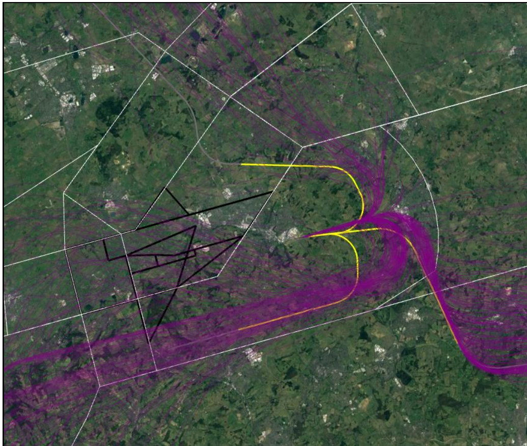
Figure 38: Existing departure swathes (purple) and the E SID Group 4 illustrative centrelines (yellow) from Luton's Easterly runway
