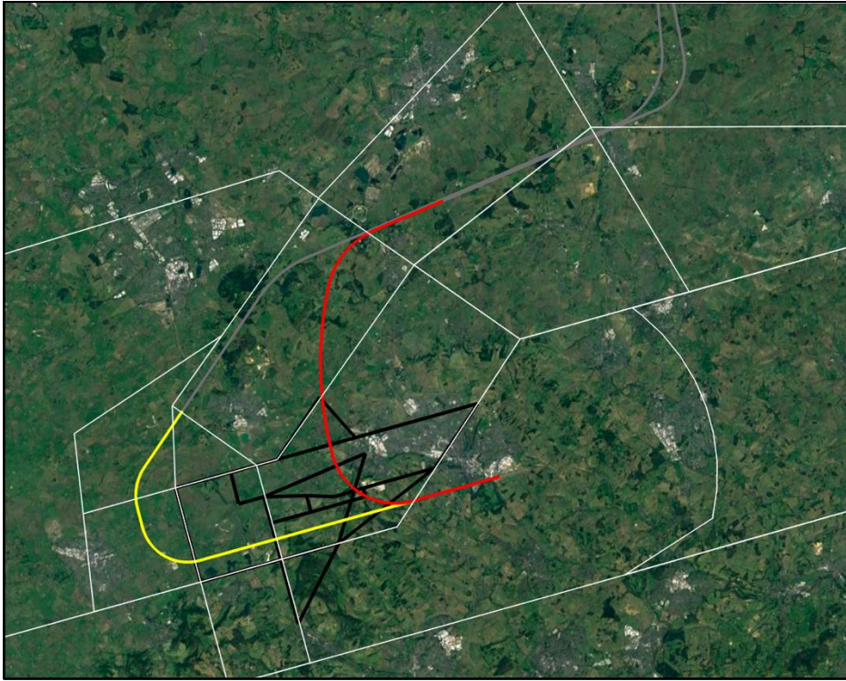
Figure 50: E Arrival Option 4 (Period 1) approach transition (yellow) with RNP-AR arrival (red)
