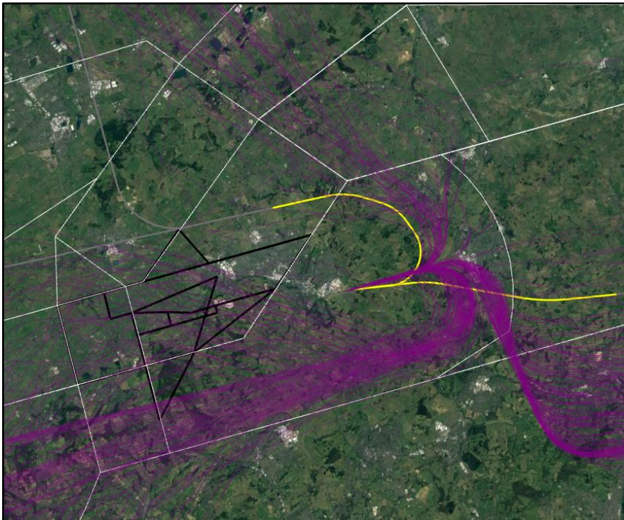
Figure 41: Existing departure swaths (purple) and the E SID Group 6 Period 2 illustrative centrelines (yellow) from Luton's Easterly runway
