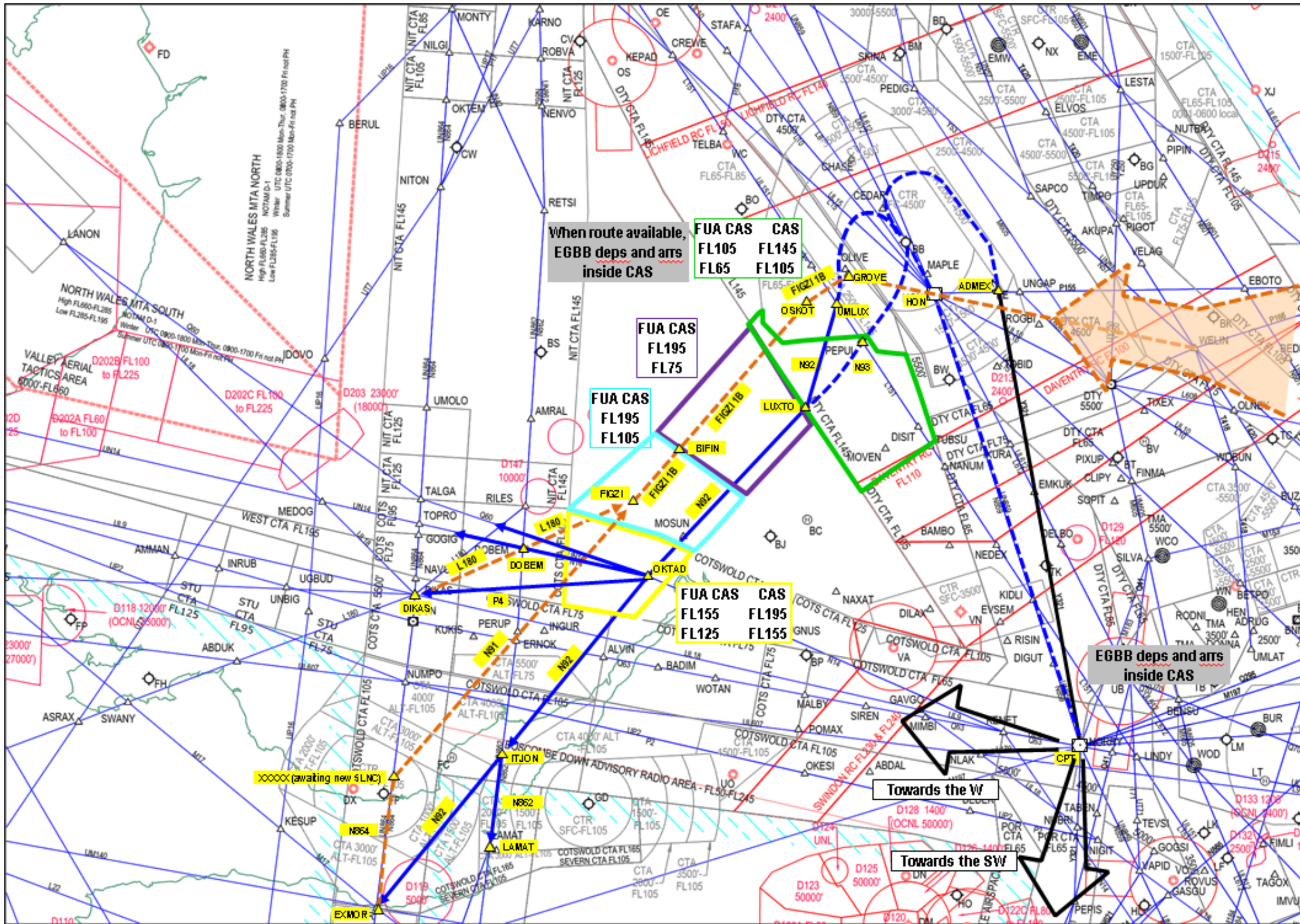
Figure 2: Proposed EGBB Traffic Flows via MOSUN (NATS' Preferred Option)
