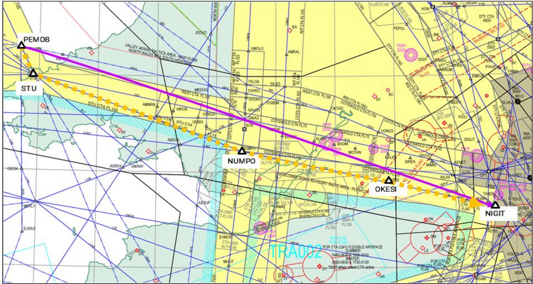
Figure 9: Proposed Eastbound ATS Route N24, PEMOB - NIGIT
