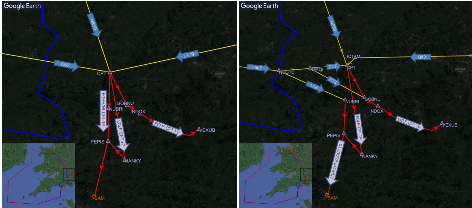
Figure 26 Current arrival connectivity and procedures for EGLF, EGHH, EGHJ airports (left) and proposed arrival connectivity and procedures (right)
