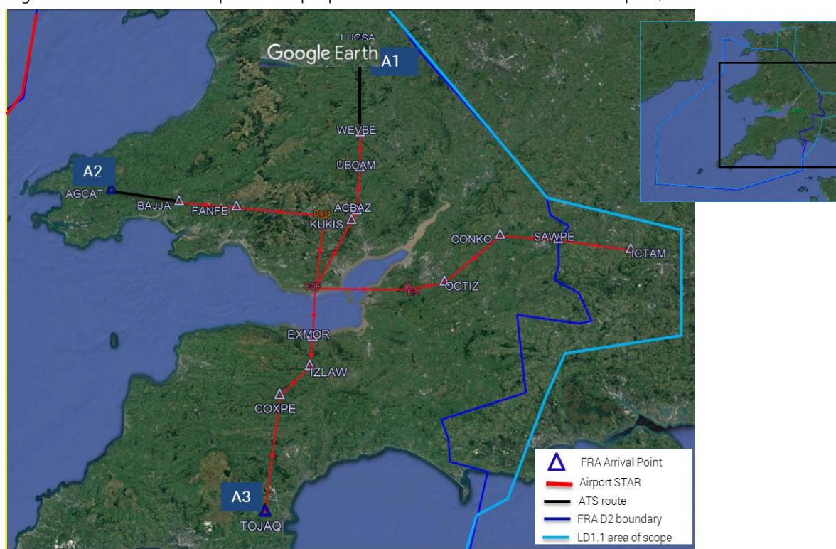
Figure 11 FRA interface: Proposed arrival structures (Cardiff Airport)
