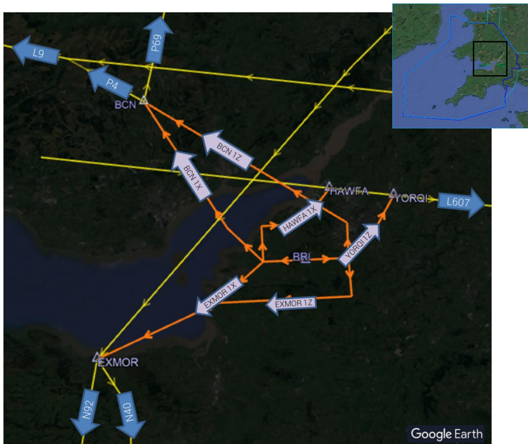
Figure 16 Bristol Airport: Proposed departure procedures and connectivity
