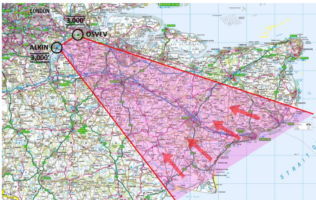
Figure 24 – Transition Arrival South
