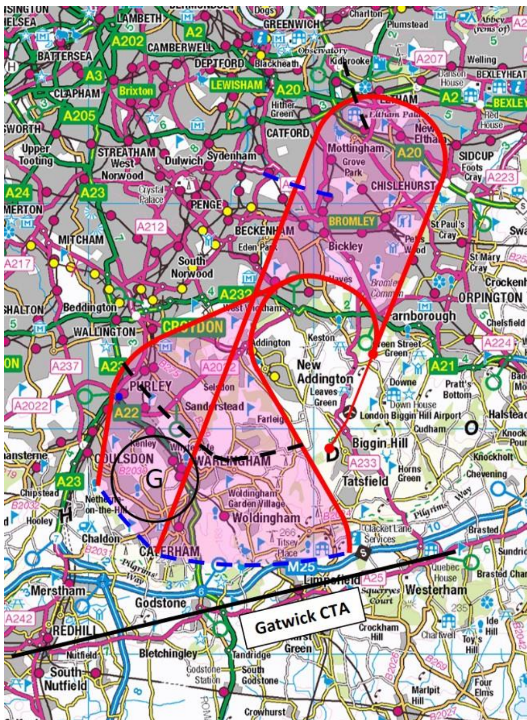
Figure 18 – Runway 03 Departures South 1
