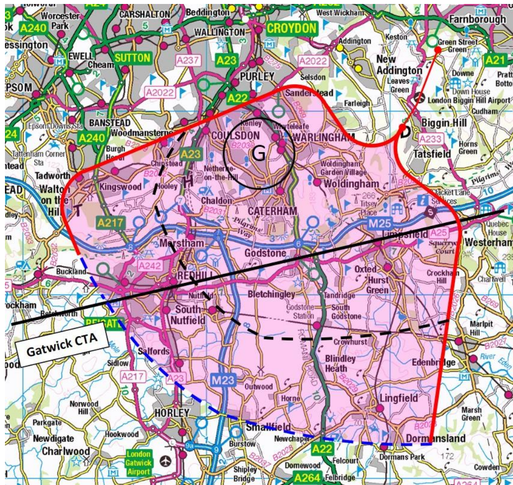
Figure 8 – Runway 21 South 1
