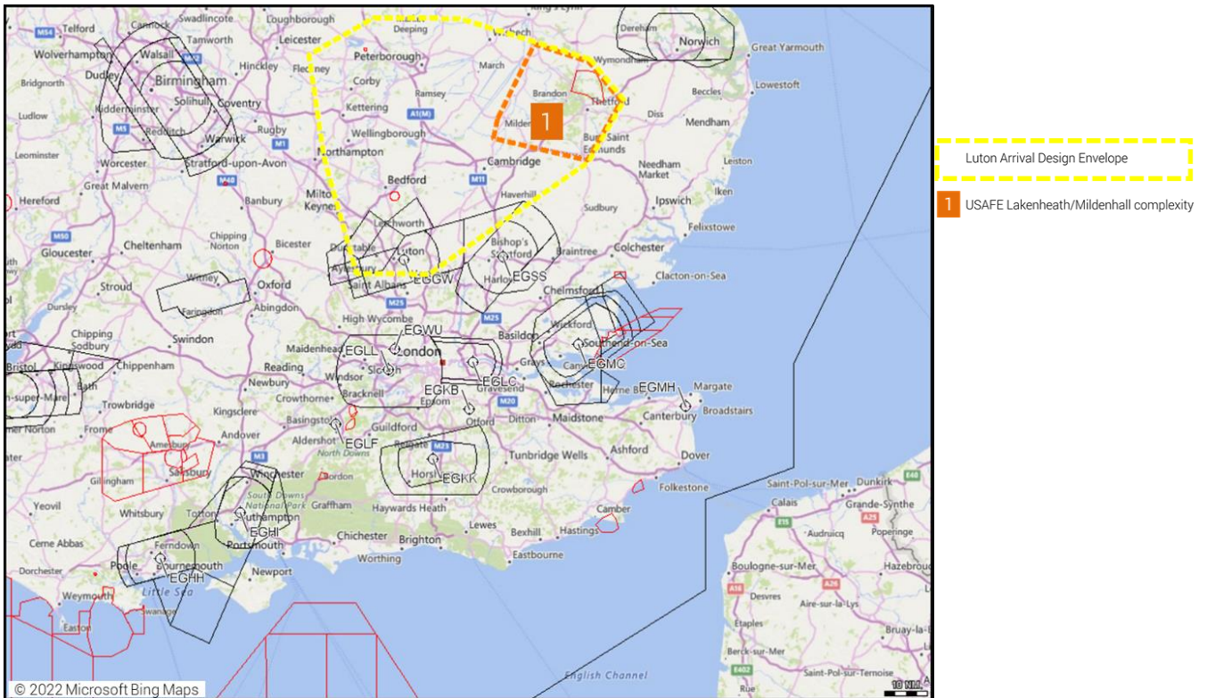
Figure 3 Luton Design Envelope and design constraints – post engagement and SME development
