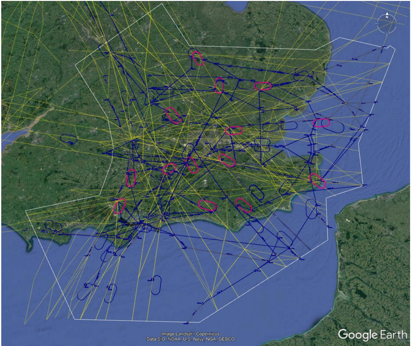
Figure 3 LTMA Airport STARs, terminal holds and ATS route connectivity 14
