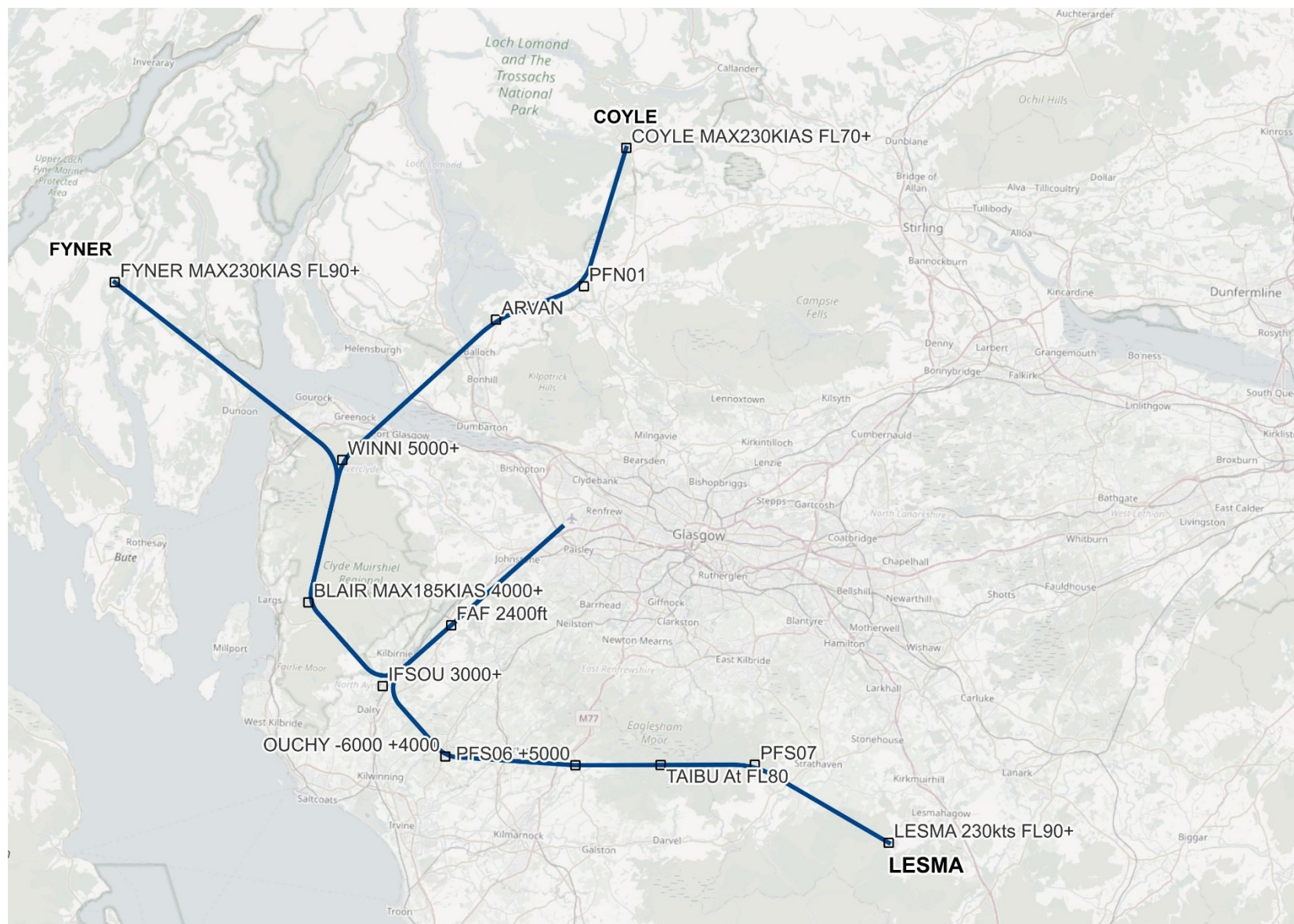
Figure 8 Runway 05 RNAV 1 (DME/DME or GNSS) arrival transitions and approach procedures (does not show missed approach procedures)
