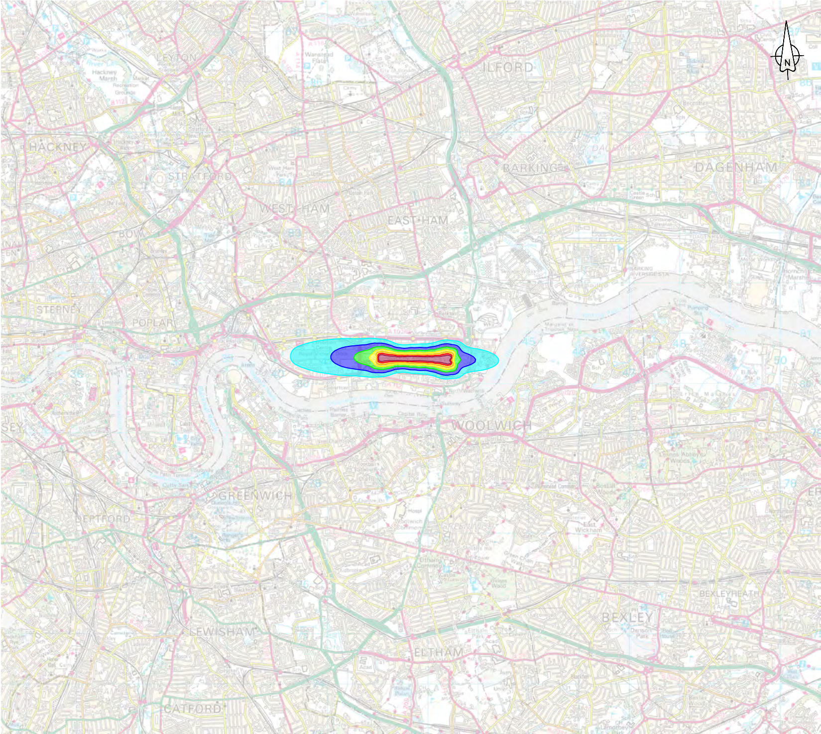
Figure 11 Average Summer Night Noise Contours 2038 With Change (Year 12)
