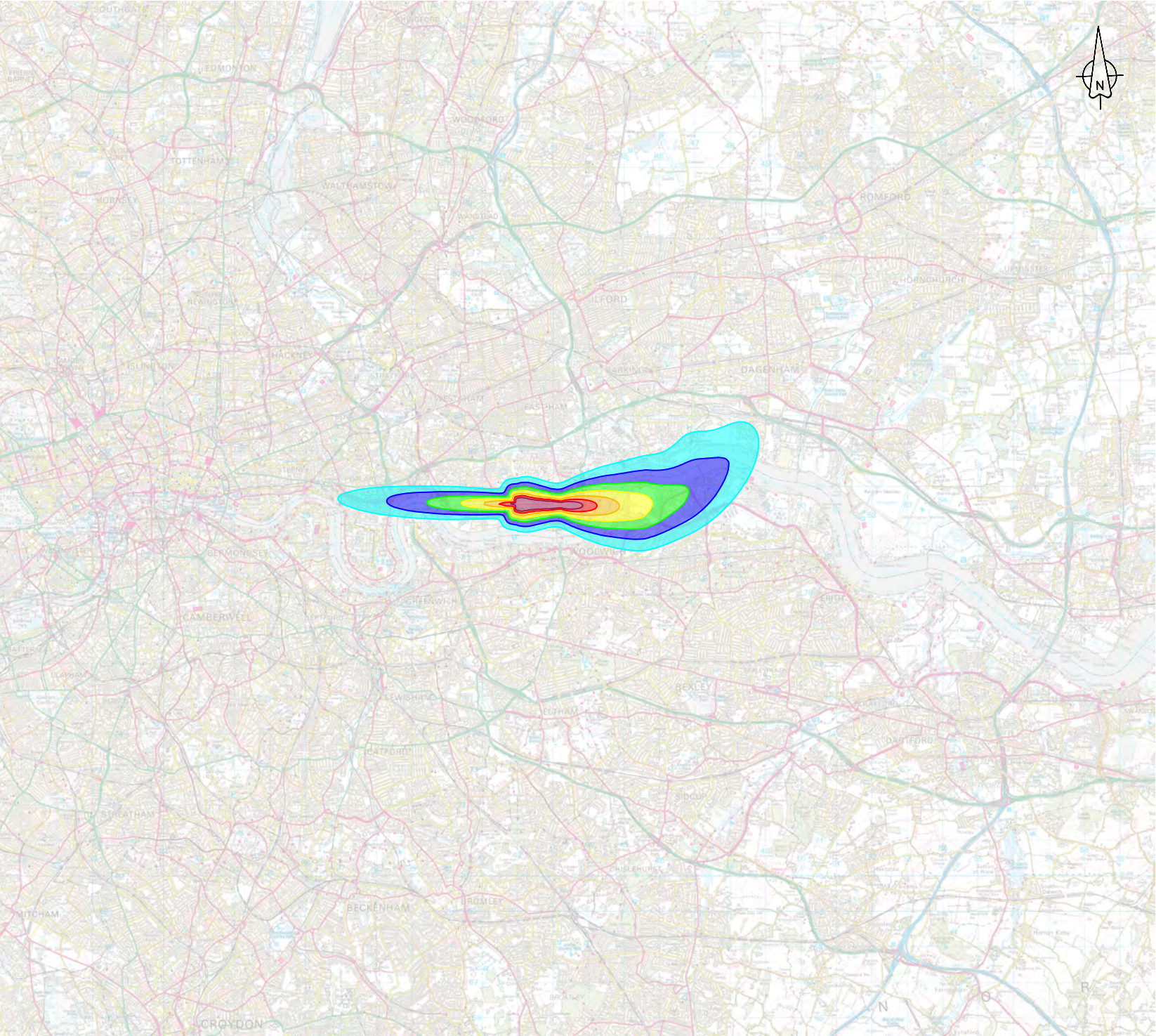
Figure 28 Easterly Mode Summer Day Noise Contours 2027 No Change (Year 1)
