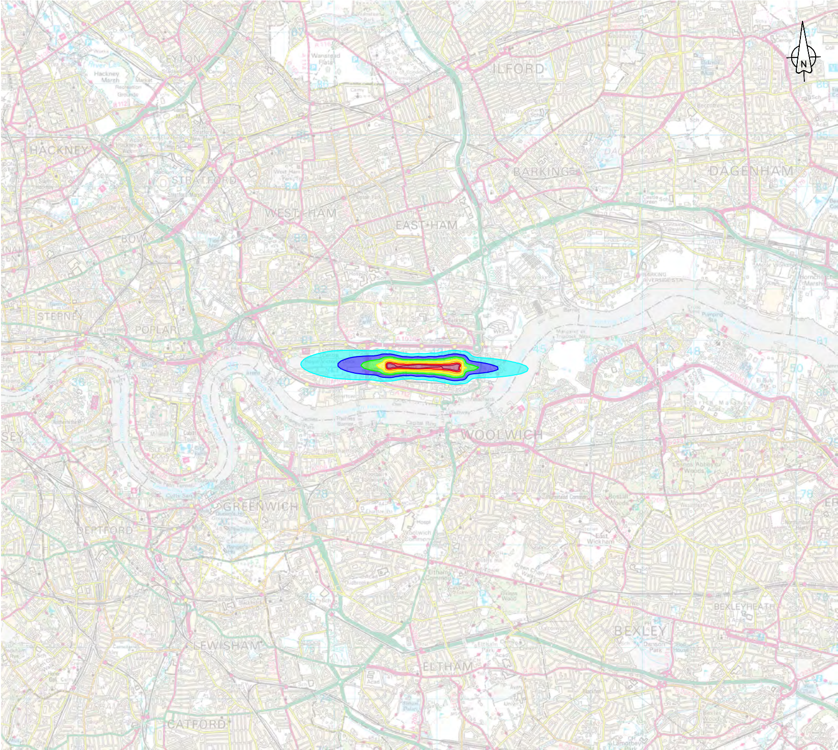
Figure 07 Average Summer Night Noise Contours 2024 Actual Average Modal
