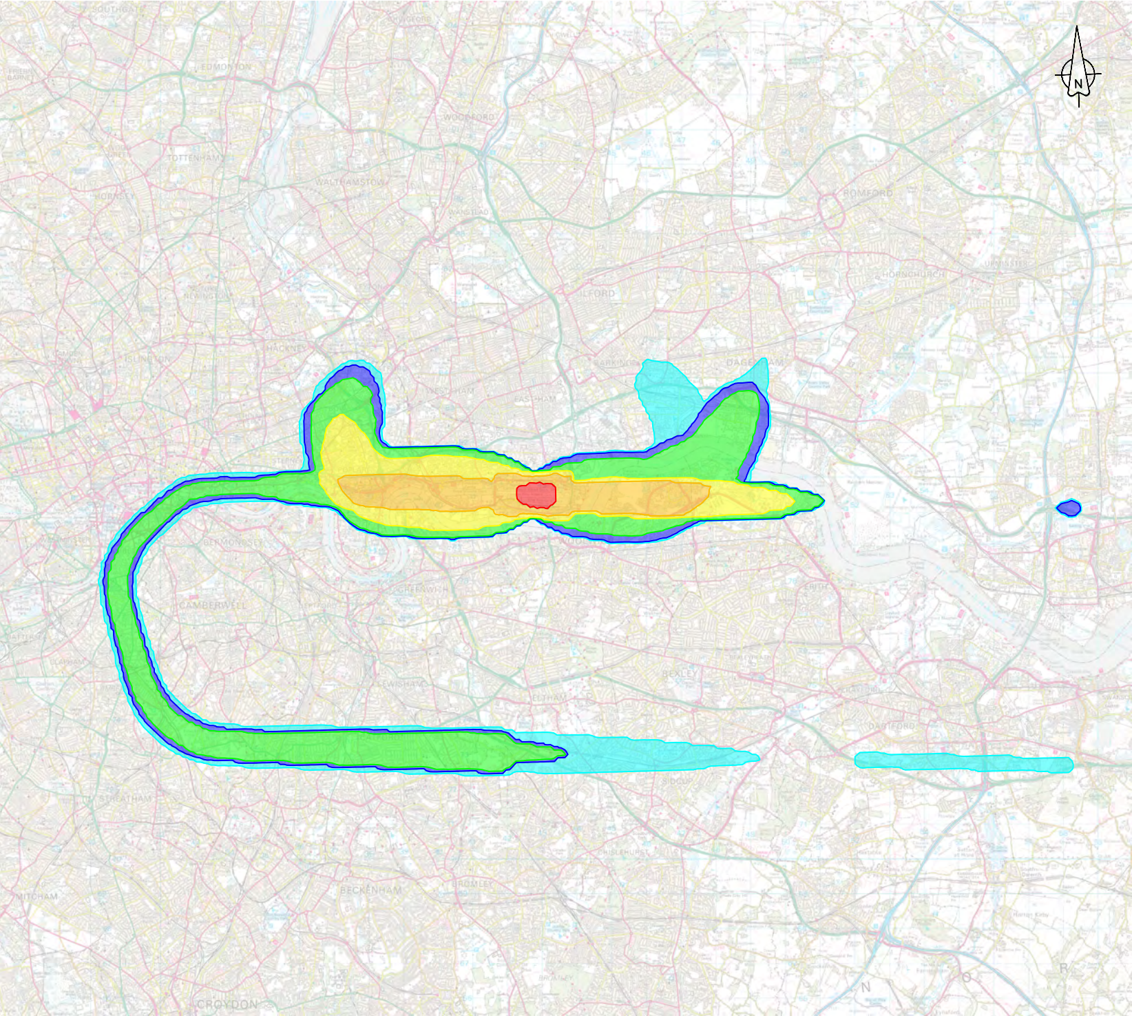
Figure 16 Average Summer Day N65 Noise Contours 2038 With Change (Year 12)
