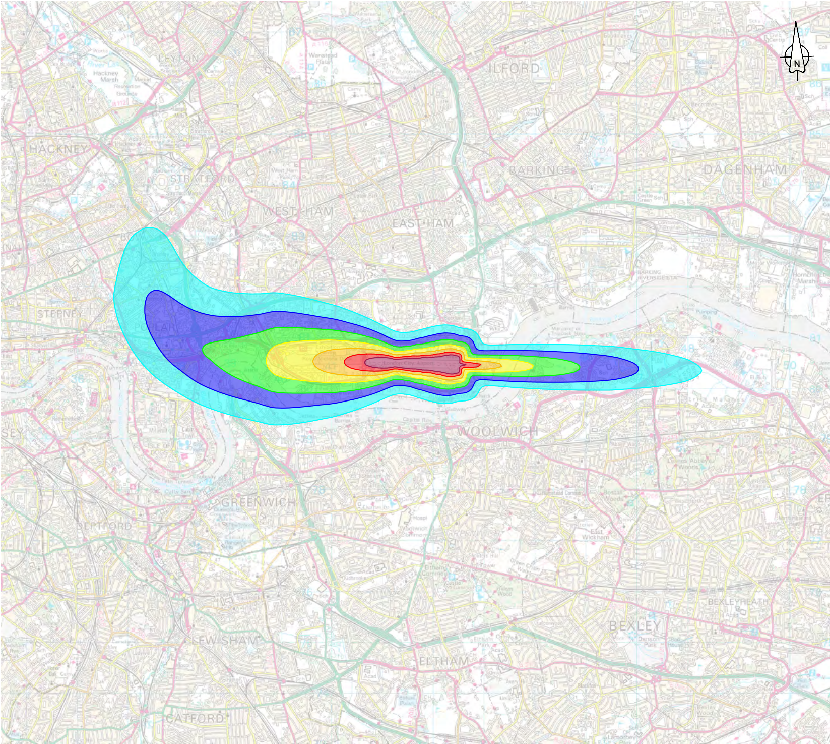
Figure 17 Westerly Mode Summer Day Noise Contours 2024 Actual
