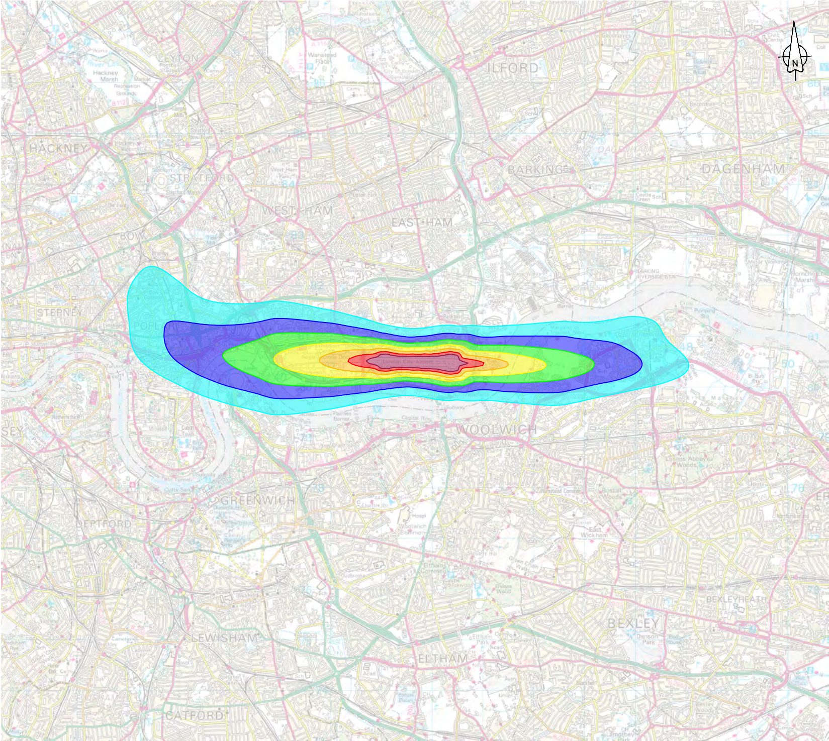
Figure 02 Average Summer Day Noise Contours 2024 Actual Average Modal
