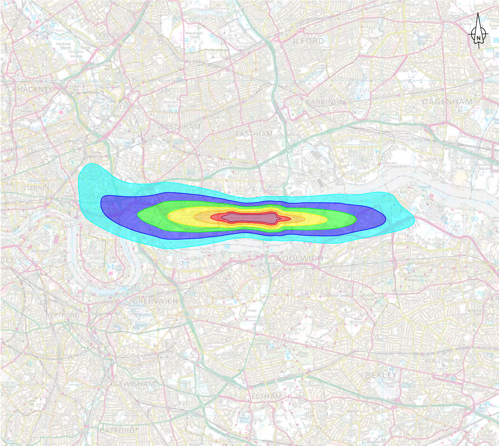
Figure 44 Summer Day Operating Hours Noise Contours 2027 With Change (Year 1)
