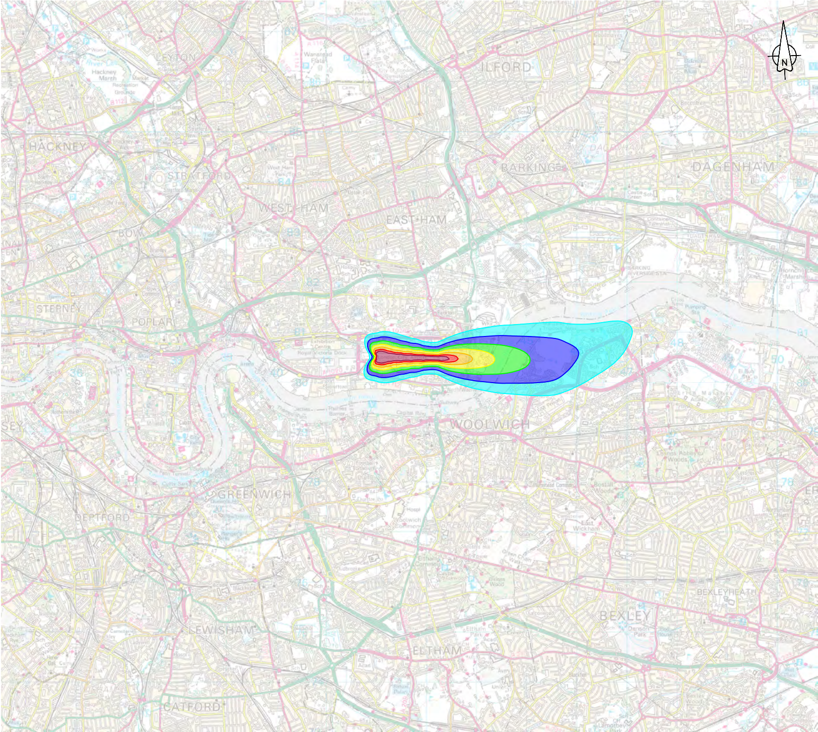
Figure 34 Easterly Mode Summer Night Noise Contours 2027 With Change (Year 1)
