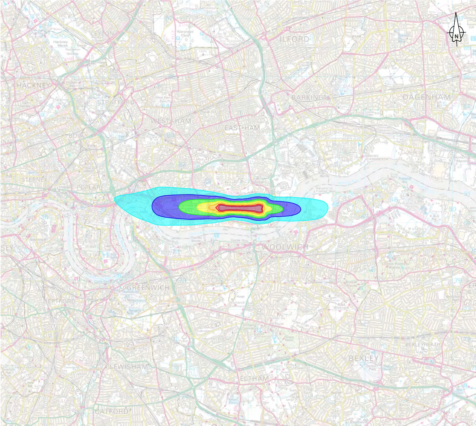
Figure 08 Average Summer Night Noise Contours 2027 No Change (Year 1)
